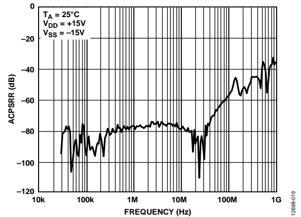
Figure 20. AC Power Supply Rejection Ratio (ACPSRR) vs. Frequency, \pm 15 V Dual Supply
