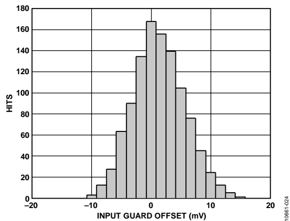
Figure 24. Distribution of Input Guard Offset Voltage V_{OLs} ( V_{INPT} - V_{SUM} )
