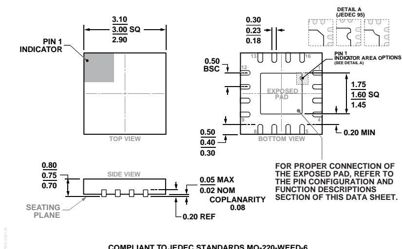
Figure 34. 16-Lead Lead Frame Chip Scale Package [LFCSP]
