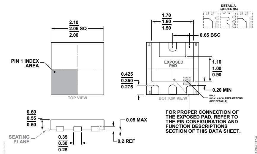
Figure 47. 6-Lead Lead Frame Chip Scale Package [LFCSP] 2.05 mm × 2.05 mm Body and 0.55 mm Package Height (CP-6-7)
