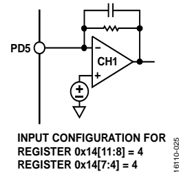
Figure 25. PD5 Connection with Register 0x14, Bits[11:8] and Bits[7:4] = 4 for the WLCSP
