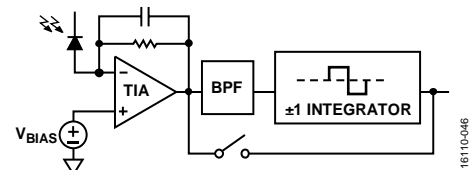
Figure 47. TIA/BPF/Integrator Block Diagram
