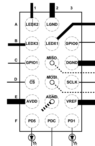
Figure 38. ADPD1081 Connection and PCB Layout Diagram, Dashed Line Traces from Blind Vias (Top View), 16-Ball WLCSP
