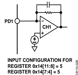
Figure 26. PD1 Connection with Register 0x14, Bits[11:8] and Bits[7:4] = 5 for the WLCSP
