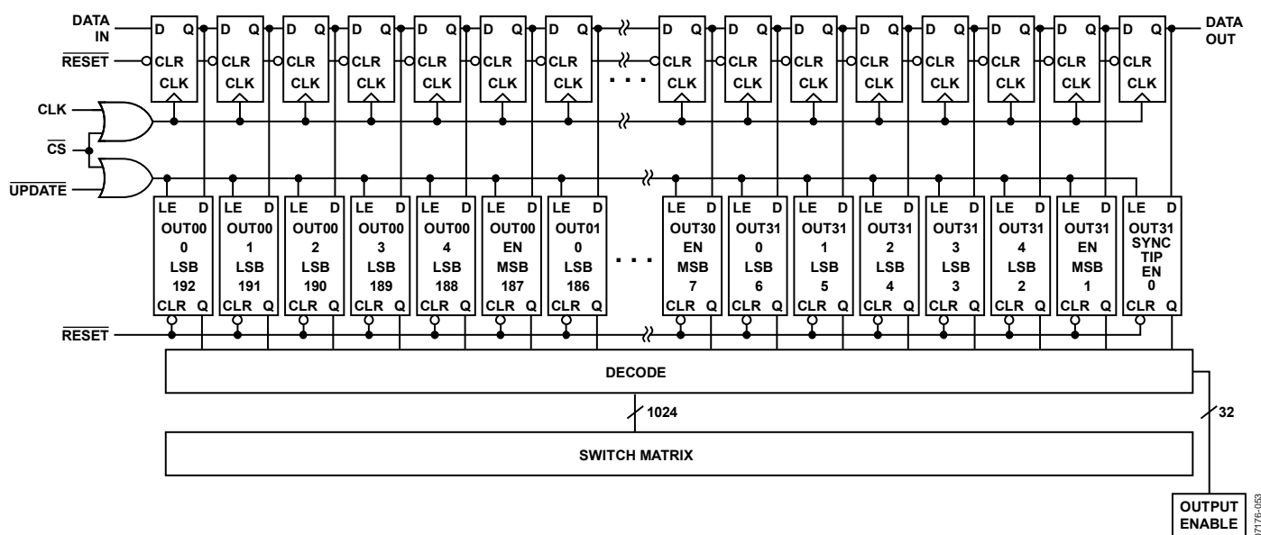
Figure 6. Logic Diagram
