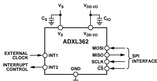
Figure 44. INT1 Pin as the Input for the External Clock
