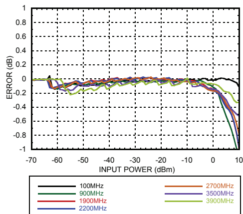
Reading Error for LTE 20MHz wrt CW Response @ +25 °C [1]
