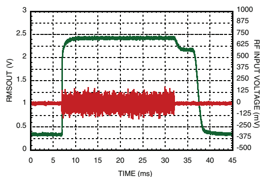
Figure 10. Residual Ripple for 1900 MHz LTE @ SCI=1111
