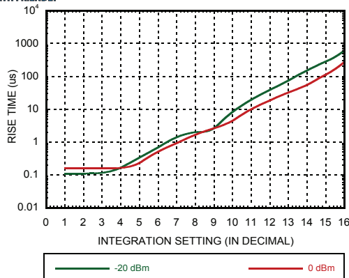
Figure 4. Rise Time [2] vs. SCI Setting over Input Power
