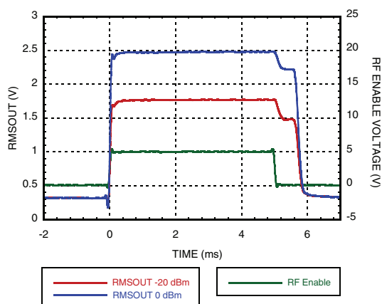
RMSOUT Output Response with SCI = 1100 @ 1900 MHz [2]
