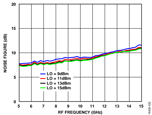
Figure 20. Noise Figure vs. RF Frequency at Various LO Power Levels, TA = 25°C
