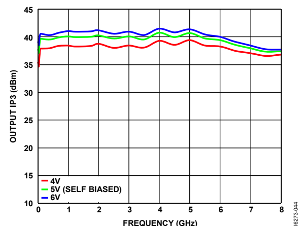
Figure 44. Output IP3 vs. Frequency for Various V_{GG2} Values, V_{DD} = 12 V, V_{GG1} = GND , P_{OUT}/Tone = 10 dBm
