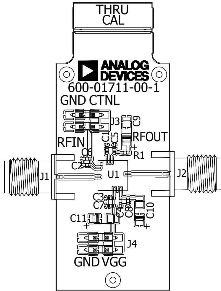
Figure 70. Evaluation PCB
