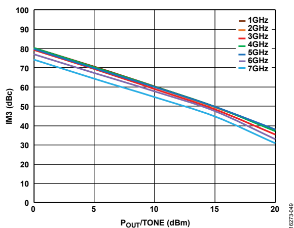
Figure 49. IM3 vs. P_{OUT}/Tone , V_{DD} = 10 V, V_{GG2} = Open , V_{GG1} = GND
