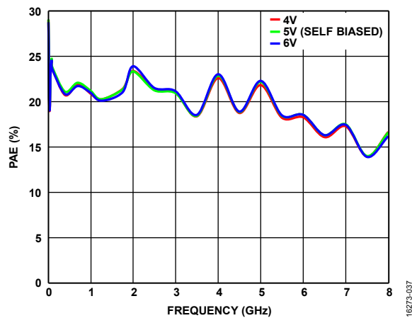
Figure 37. PAE vs. Frequency for Various V_{GG2} Values, V_{DD} = 12\text{ V} , V_{GG1} = \text{GND} , PAE Measured at P_{SAT}
