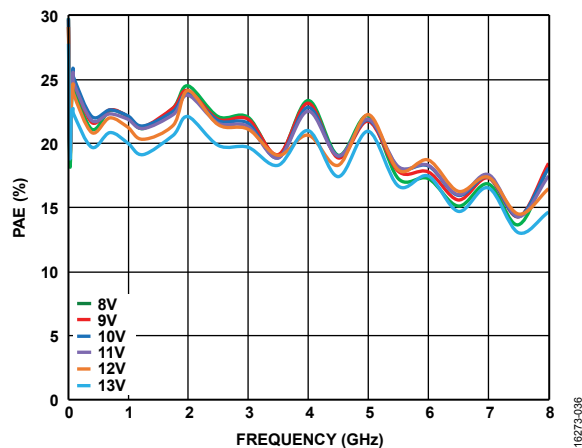
Figure 36. PAE vs. Frequency for Various Supply Voltages ( V_{DD} ), V_{GG2} = \text{Open} , V_{GG1} = \text{GND} , PAE Measured at P_{SAT}
