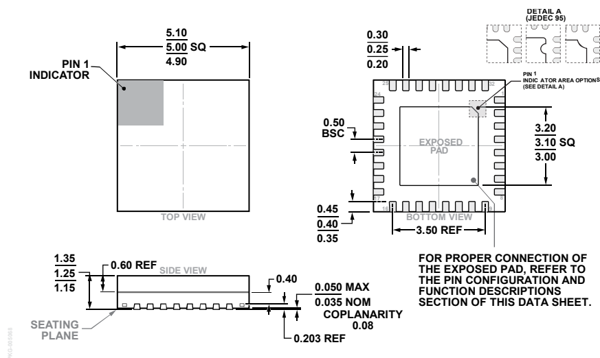
Figure 71. 32-Lead Lead Frame Chip Scale Package, Premolded Cavity [LFCSP_CAV] 5 mm × 5 mm Body and 1.25 mm Package Height (CG-32-2)
