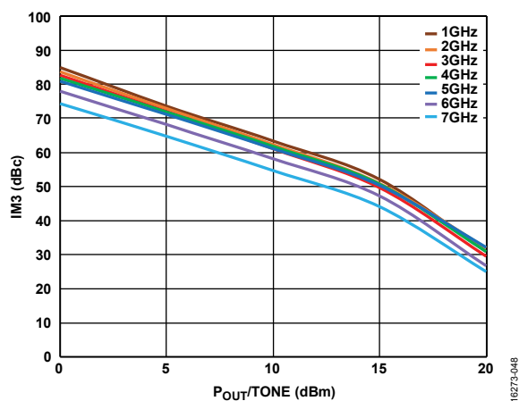
Figure 48. IM3 vs. P_{OUT}/Tone , V_{DD} = 8 V, V_{GG2} = Open , V_{GG1} = GND
