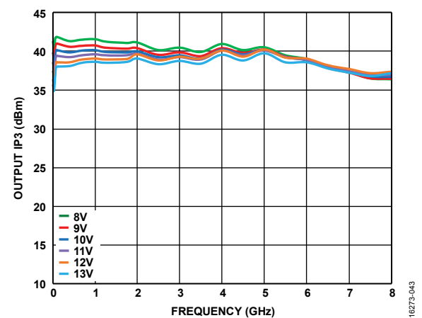
Figure 43. Output IP3 vs. Frequency for Various Supply Voltages ( V_{DD} ), V_{GG2} = Open , V_{GG1} = GND , P_{OUT}/Tone = 10 dBm
