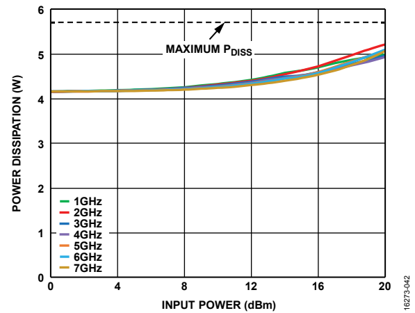
Figure 42. Power Dissipation vs. Input Power at T_A = 85^\circ\text{C} , V_{DD} = 12 V, V_{GG1} = GND , V_{GG2} = Open
