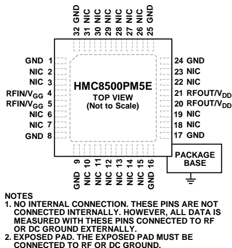
Figure 2. Pin Configuration
