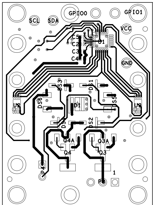
Figure 13. EVAL-ADPD2140Z Evaluation Board Layout
