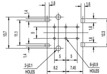
PIERCING PLAN
