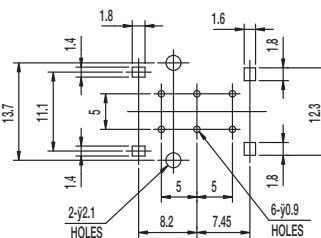
PIERCING PLAN
