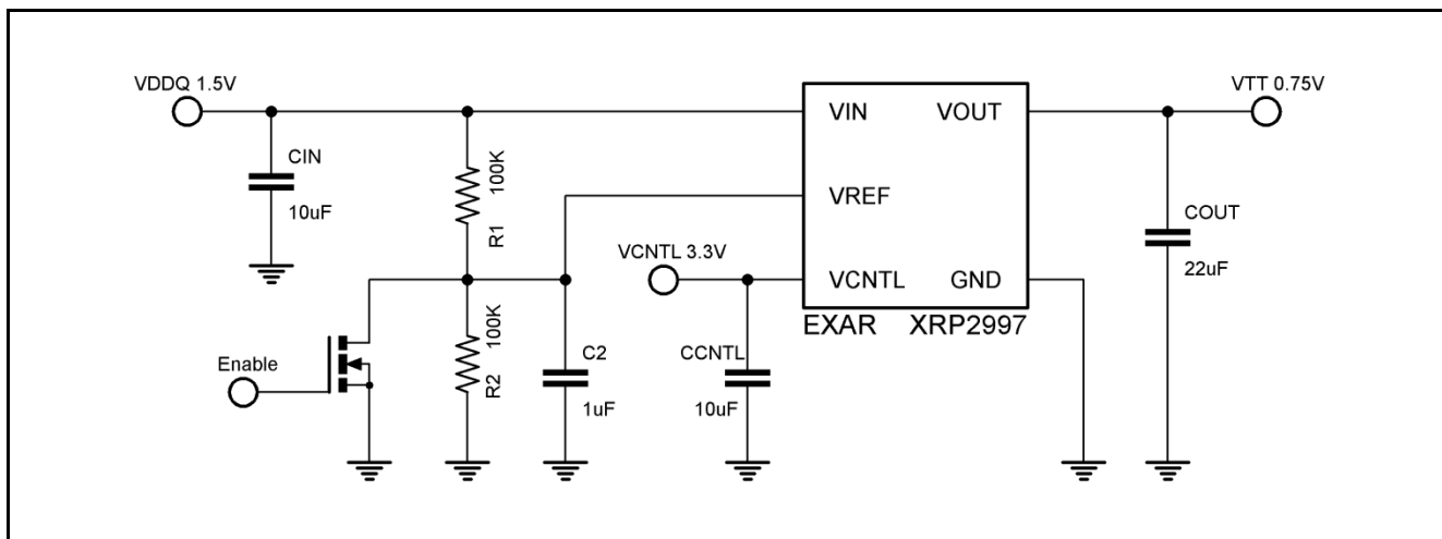
Fig. 1: XRP2997 DDRIII V TT Application Diagram
