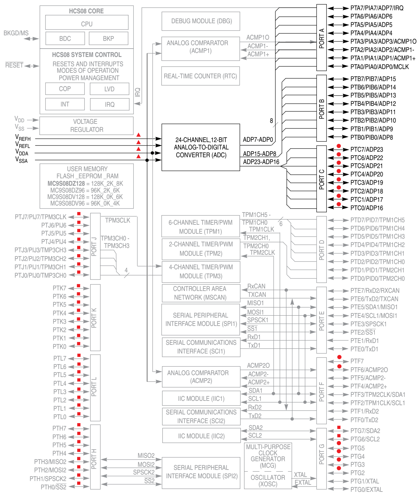
Figure 10-1. MC9S08DZ128 Block Diagram with ADC Highlighted
