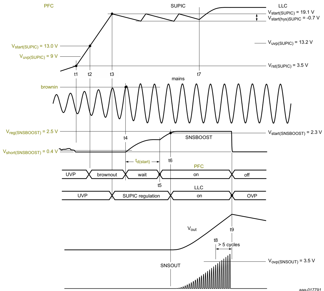
Fig 24. System protection
