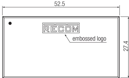
Dimension Drawing Single Wired (mm) 12-48Vout available from Dec/2018
