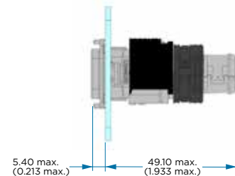
Universal Unshielded Accessory
