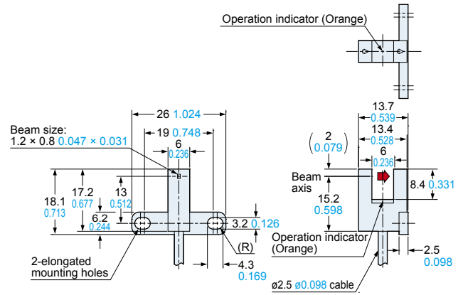
PM-T45□ Sensor
