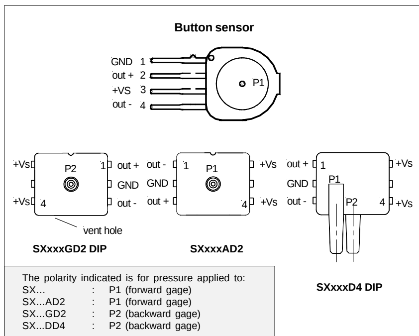
Button sensor or "N" package
