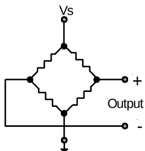
Button sensor or "N" package
