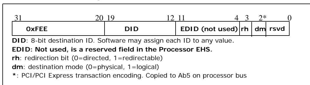
Figure 5-13. XAPIC Address Encoding
