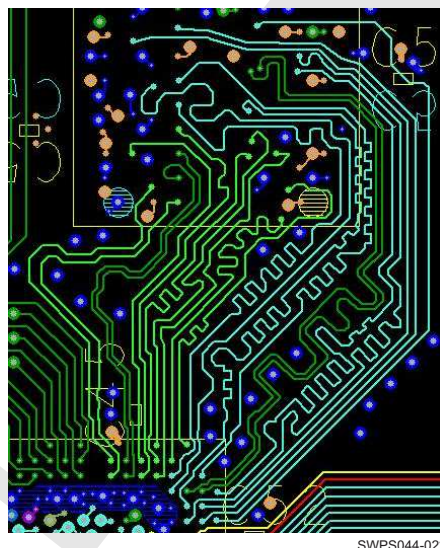
Figure 8-20. Routing DQ0/2 (L2)
