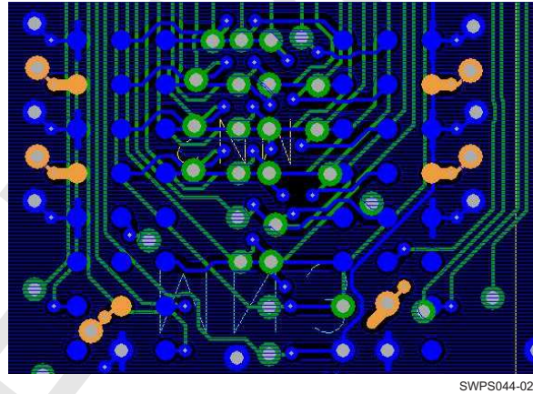
Figure 8-22. Command-Address Routing L1/L2
