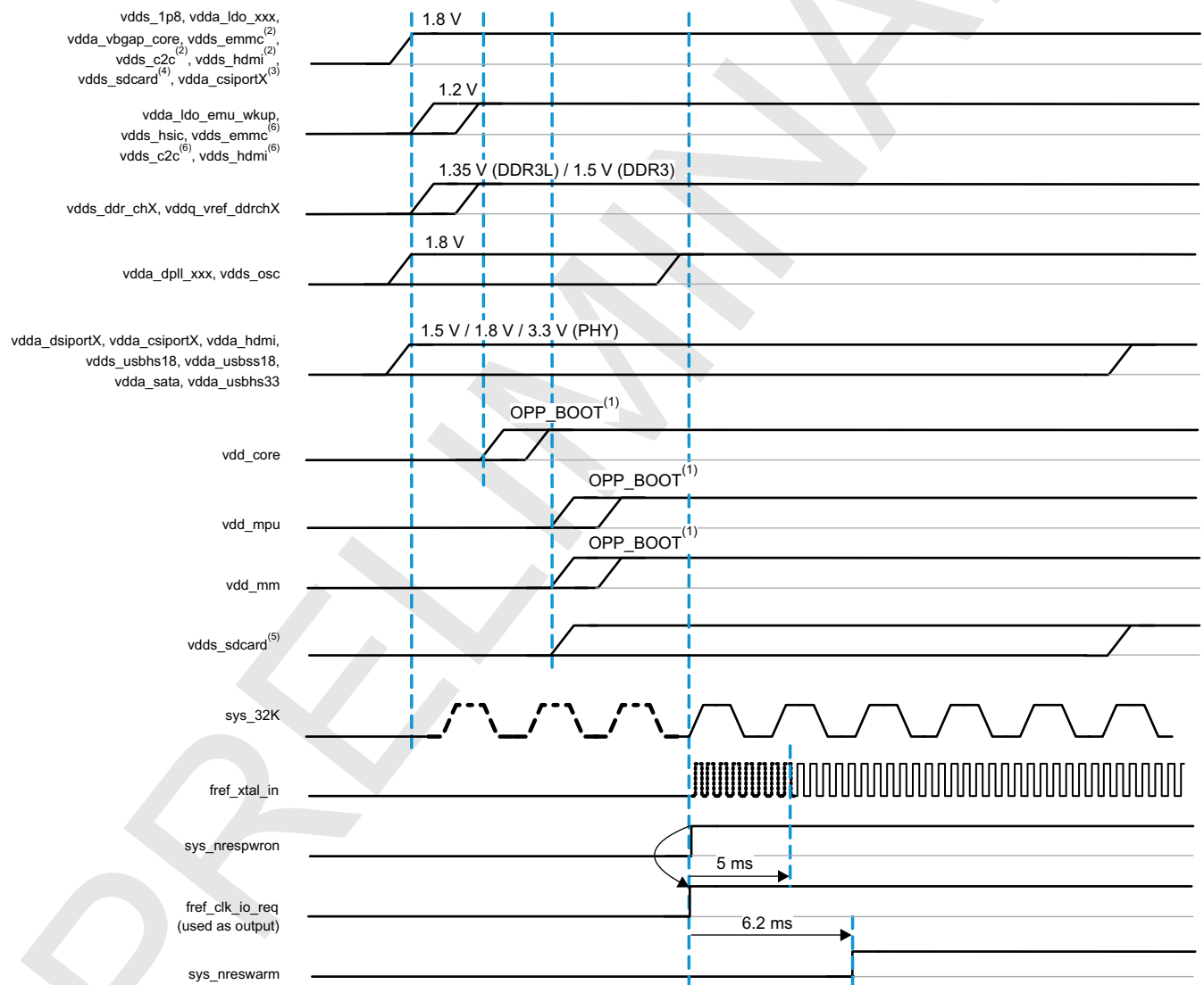
Figure 3-2. Power-Up Sequence
