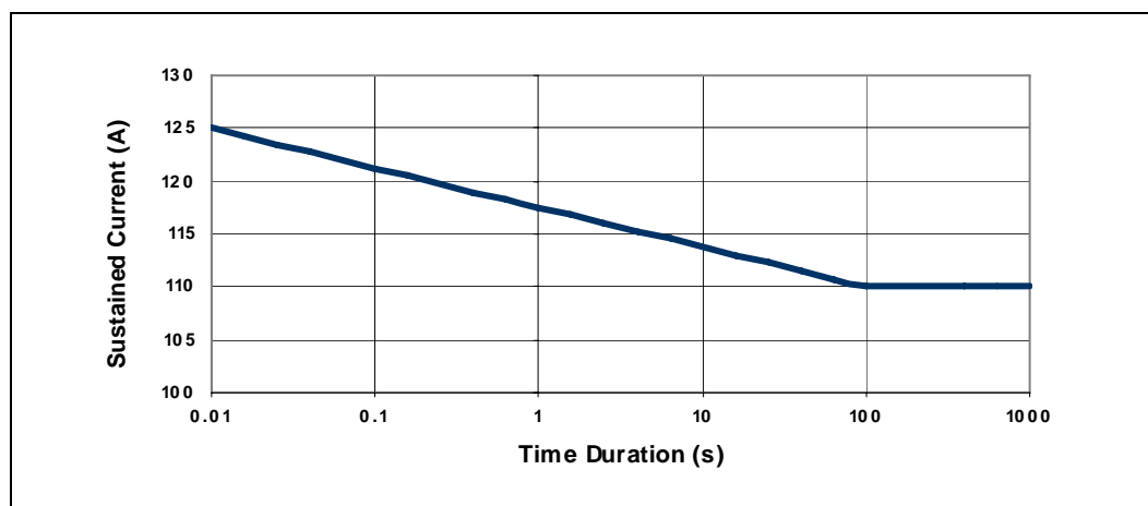
Figure 2-3. Quad-Core Intel® Xeon® Processor X5400 Series Load Current versus Time
