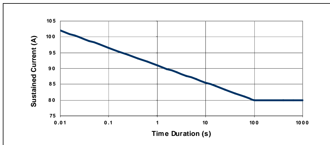
Figure 2-4. Quad-Core Intel® Xeon® Processor E5400 Series Load Current versus Time
