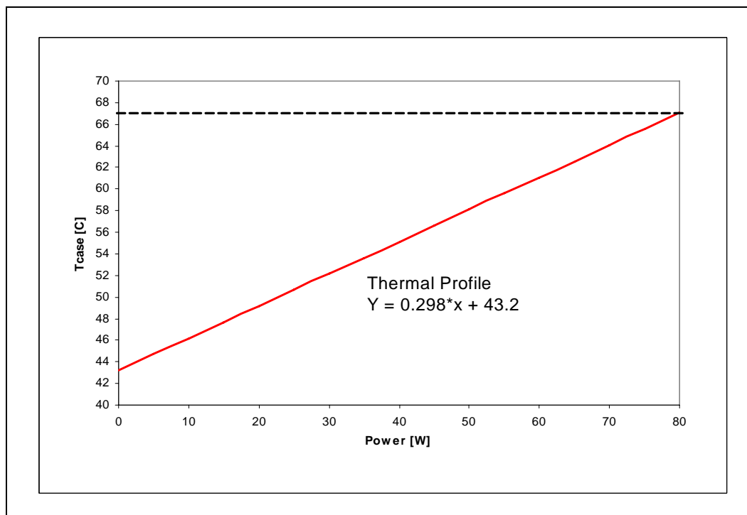
Figure 6-3. Quad-Core Intel® Xeon® Processor E5400 Series Thermal Profile
