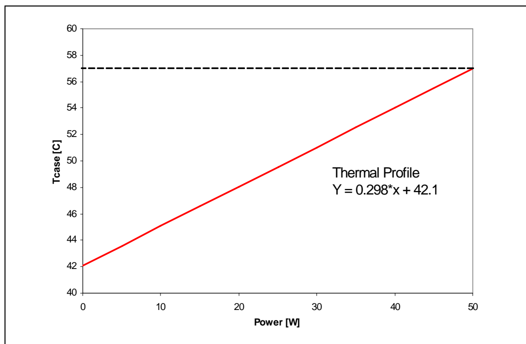
Figure 6-4. Quad-Core Intel® Xeon® Processor L5400 Series Thermal Profile
