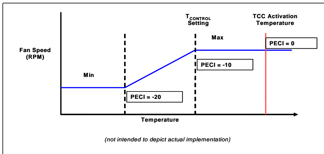
Figure 6-9. Conceptual Fan Control Diagram of PECI-based Platforms
