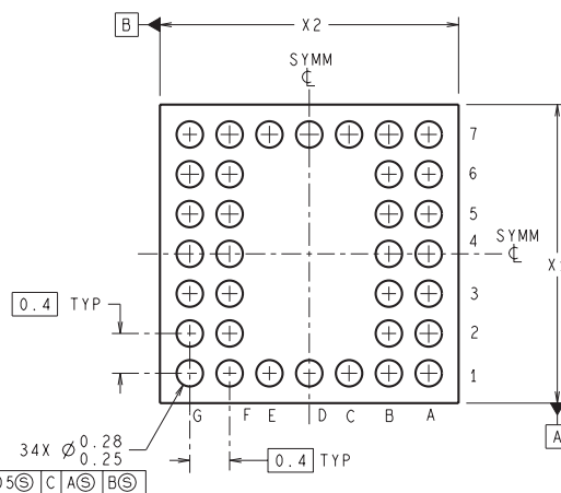
BOTTOM SIDE OF PACKAGE
