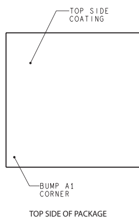
TOP SIDE OF PACKAGE
