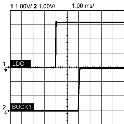
From LDO Startup to Buck 1 Startup
