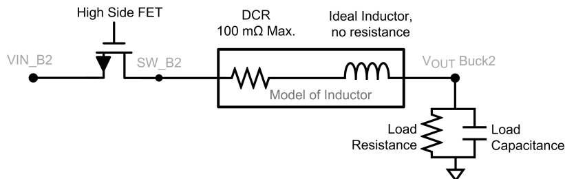
Equivalent Circuit of Bypass Operation of Buck 2 (Not Applicable to LM10506-B)
