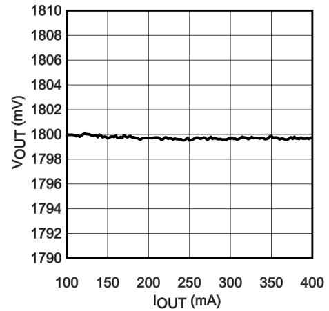
Buck 2 V_{OUT} vs. I_{OUT} V_{IN}=5.0V , V_{OUT}=1.8V
