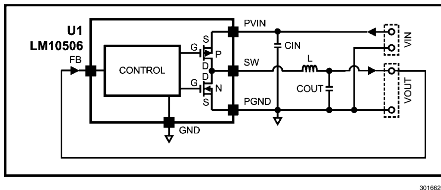
FIGURE 4. Buck Functional Diagram
