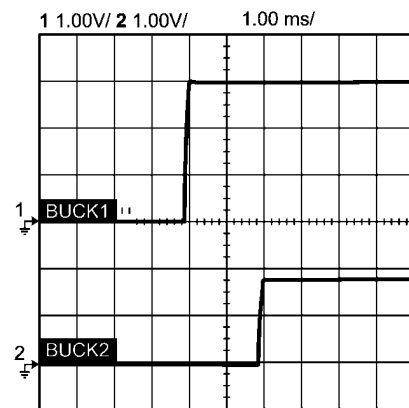
From Buck 1 Startup to Buck 2 Startup
