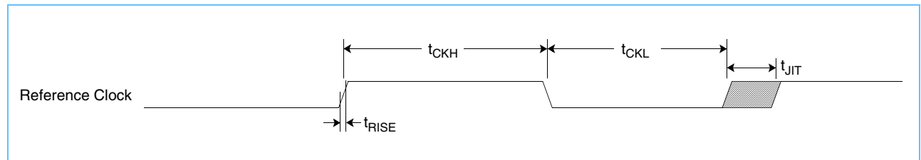
Figure 3-3. PLL Reference Clock Parameters
