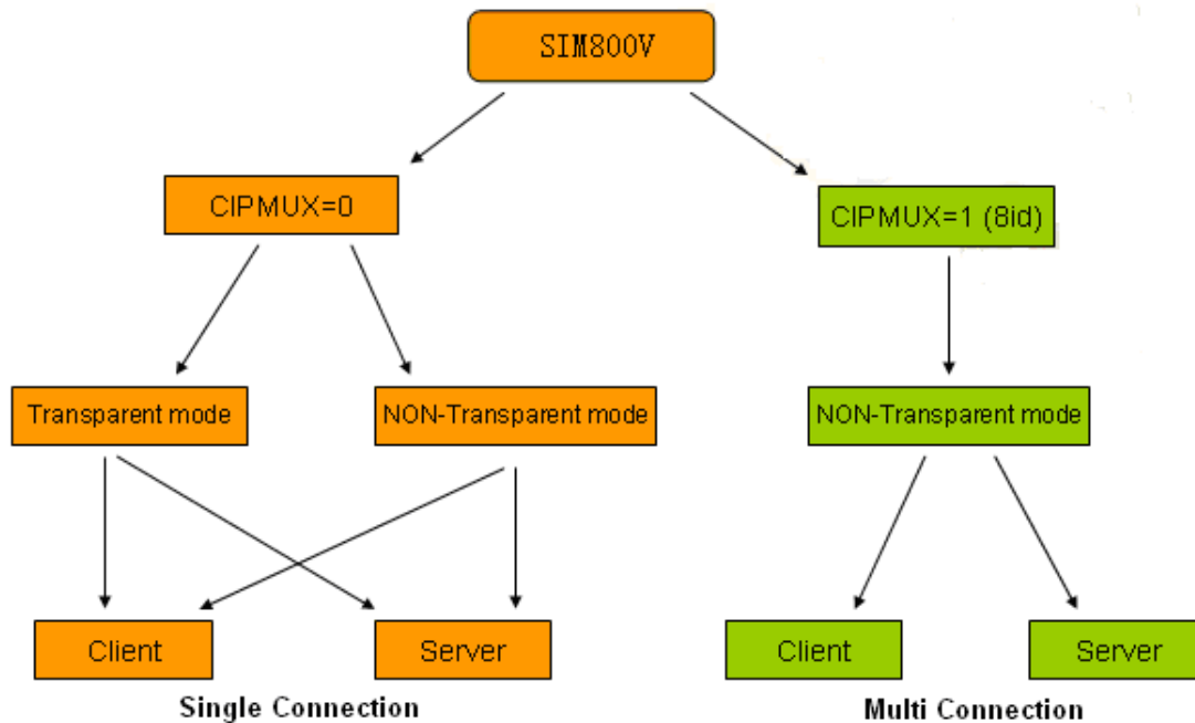
Figure1: SIM800 series TCPIP Structure
