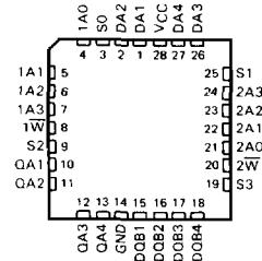
SN54AS871 . . . FK PACKAGE SN74AS871 . . . FN PACKAGE
