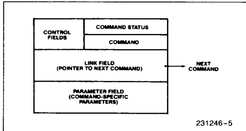
Figure 5. Action Command Format
