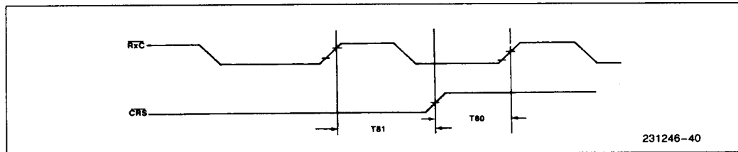
Figure 38. CRS Timing Relative to RxC
