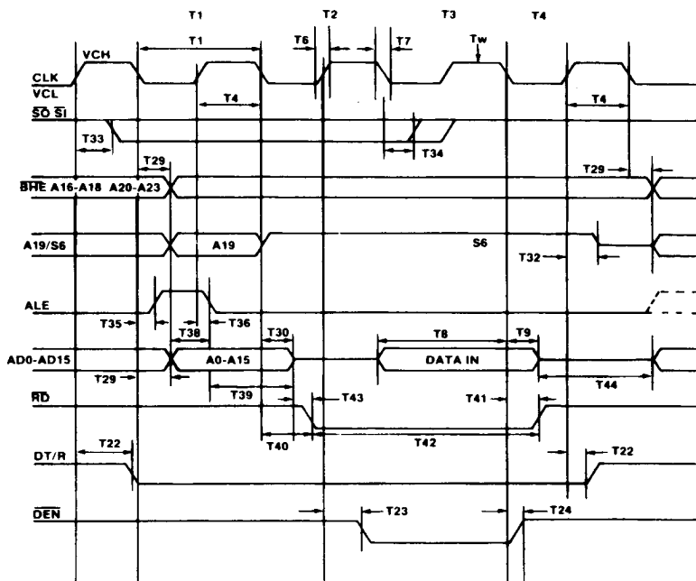
Figure 31. Read Cycle Timing
