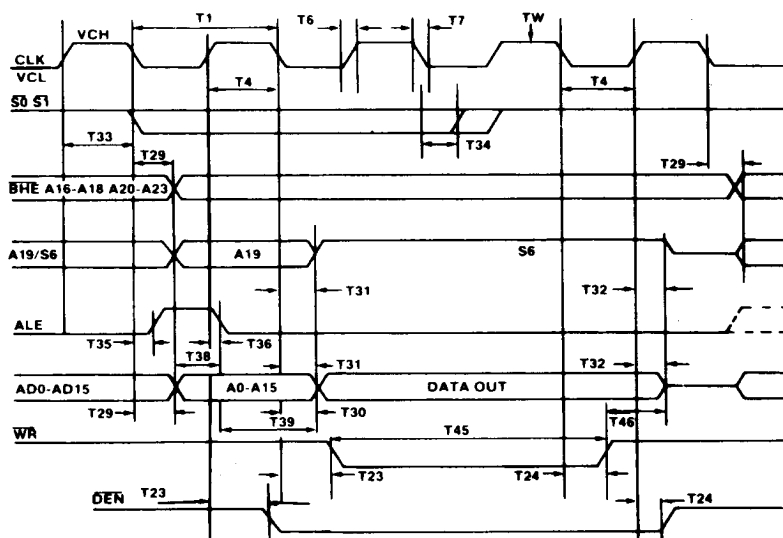
Figure 32. Write Cycle Timing
