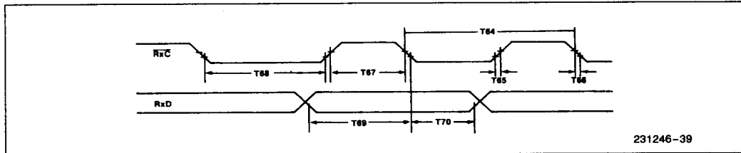
Figure 37. Rxv Timing Relative to RxC
