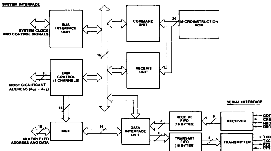
Figure 1. 82586 Functional Block Diagram
