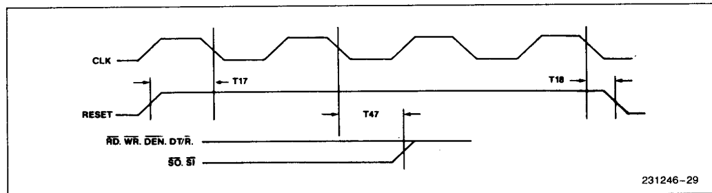
Figure 28. RESET Timing
