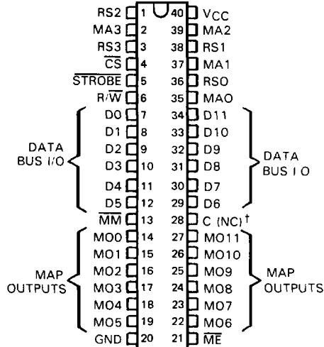
SN54LS'... JD PACKAGE SN74LS'... JD OR N PACKAGE (TOP VIEW)
